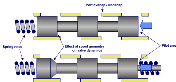
Figure 3: Modifiable parameters for spool modelling
