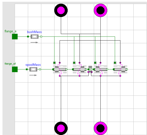
Figure 1: Power steering spool valve model
