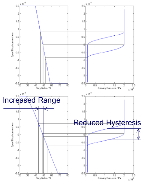
Figure 6: Increased controllability of CVT
