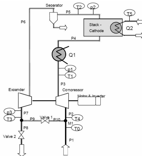
Figure 1: Sketch of the fuel cell subsystem to simulate
